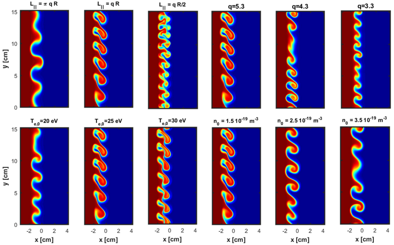
Figure 6. Snapshots of the density at the time where the initial perturbation of the unstable plasma become visible. Each frame is an individual simulation. Input parameters are as for figure 2 except that L_y = 15 cm and the input parameter is given in the titles. Red areas denote high densities and blue areas denote low densities.
